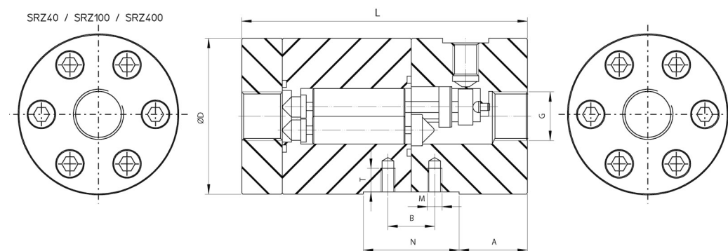
Figure 3 – Dimensional drawing SRZ compact
