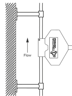
Fig. 4: Vertical Installation
